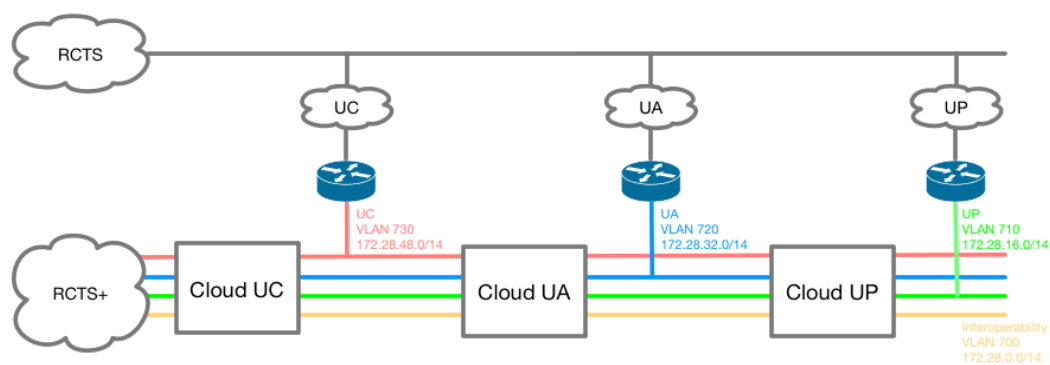
Figure 3 Cloud4IES VLANs interconnection
